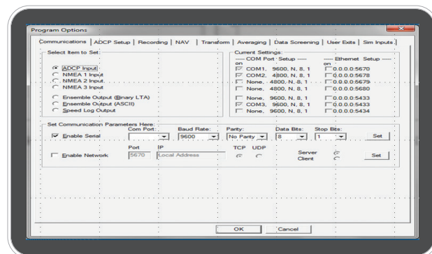
Supports real-time current profile data collection from a Sentinel V mounted on a vessel
