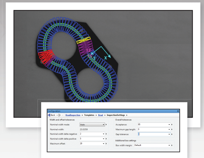
Bead Inspection
