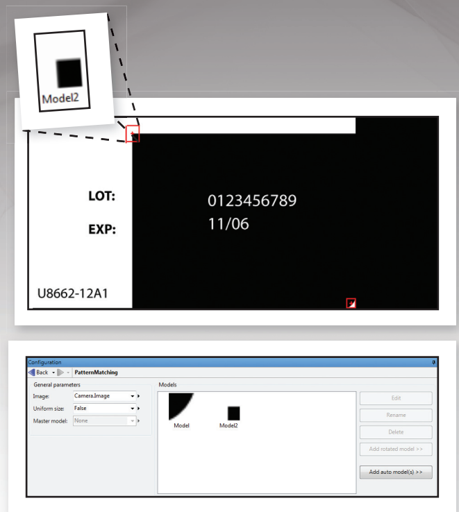
Pattern Matching
