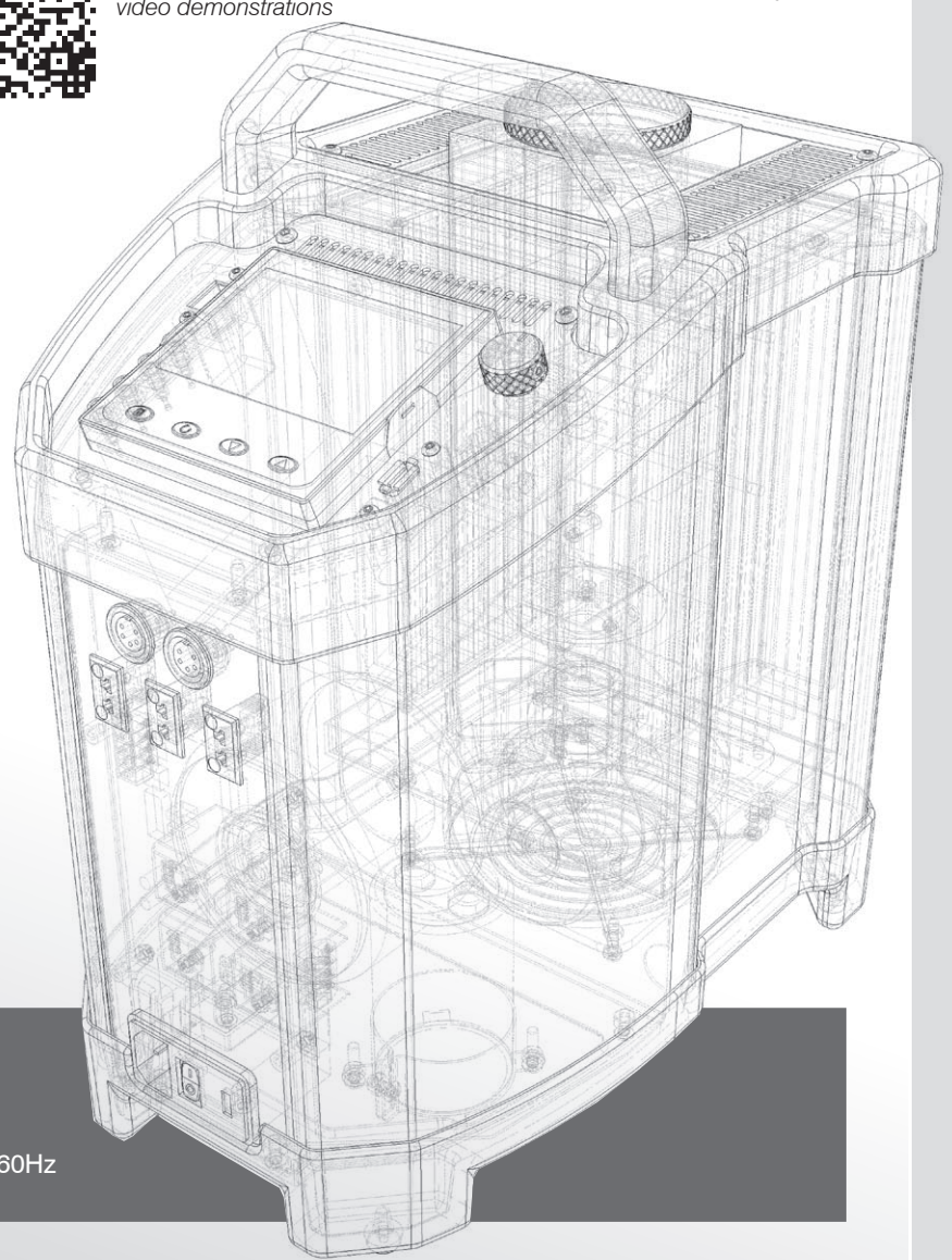
Four distributed heat/cooling zones for optimum uniformity
