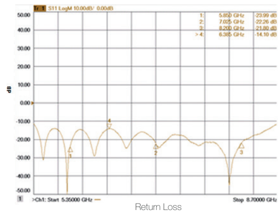
Return Loss
