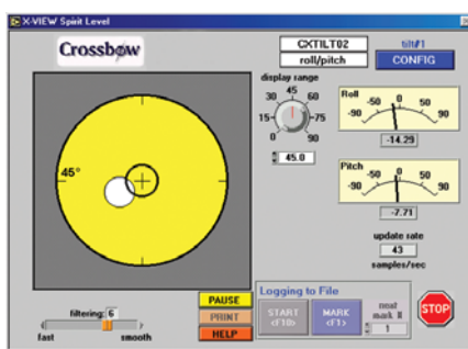
Figure 1. Development Software
