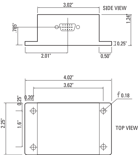
Aluminum Package
