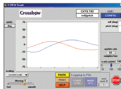
Figure 2. Development Software
