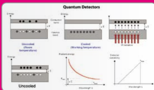
Figure 1. Operating principle of quantum detectors
